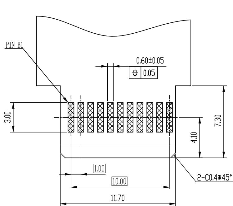
Recommended PCB Layout(±0.05)
