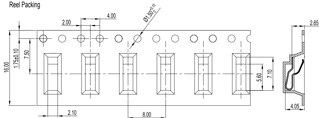
Reel Packing
