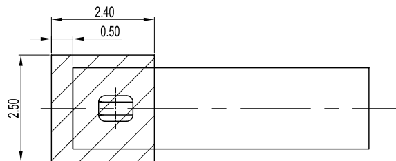
SOLDER P.C.B LAYOUT TOP VIEW
