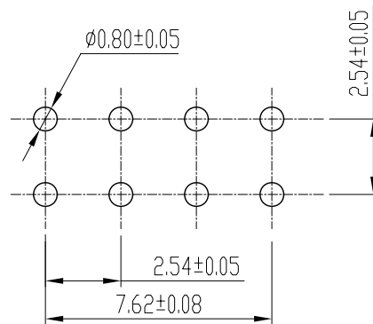
RECOMMENDED PCB LAYOUT(head)
