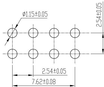
RECOMMENDED PCB LAYOUT(tail)
