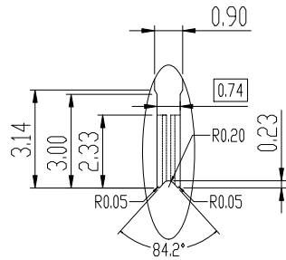
DETAIL A SCALE 5:1
